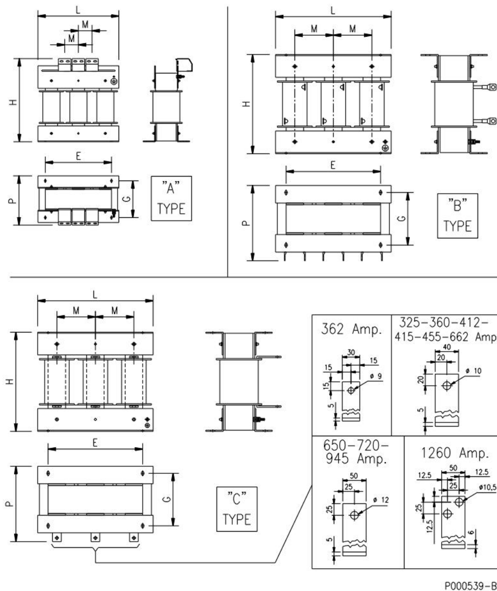
Figure 31: Mechanical features of a 3-phase reactor
