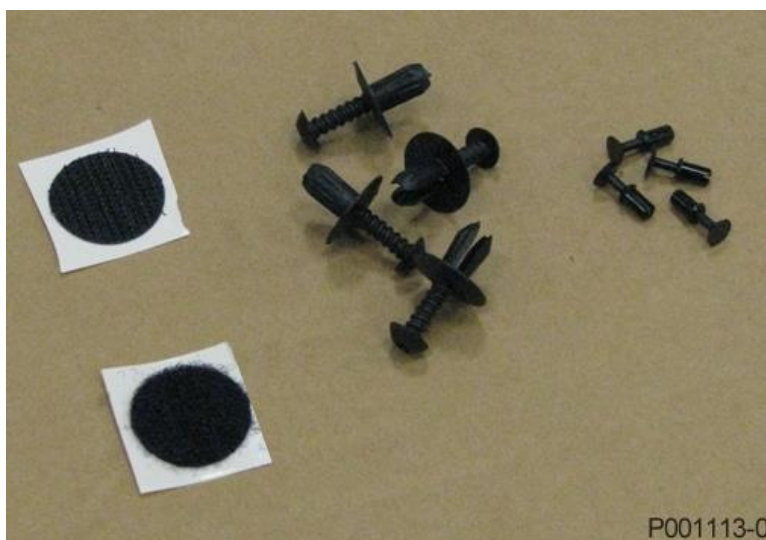
Figure 27: Velcro items to fasten the cover; fasteners to fix the junction plates; rivets to fix the bottom covers
